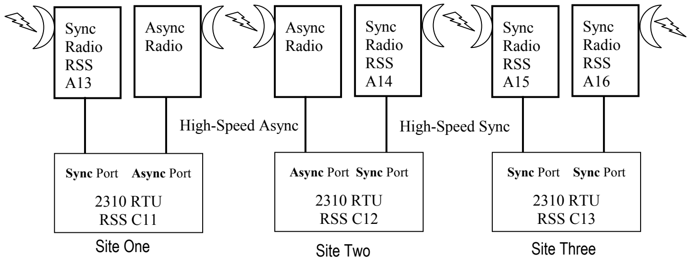
FIGURE 8. EXAMPLE OF HIGH-SPEED ASYNCHRONOUS HOP
